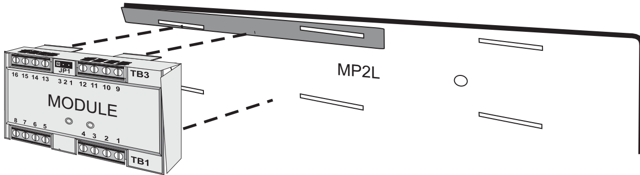
Figure 2, Mounting Module to MP2L
