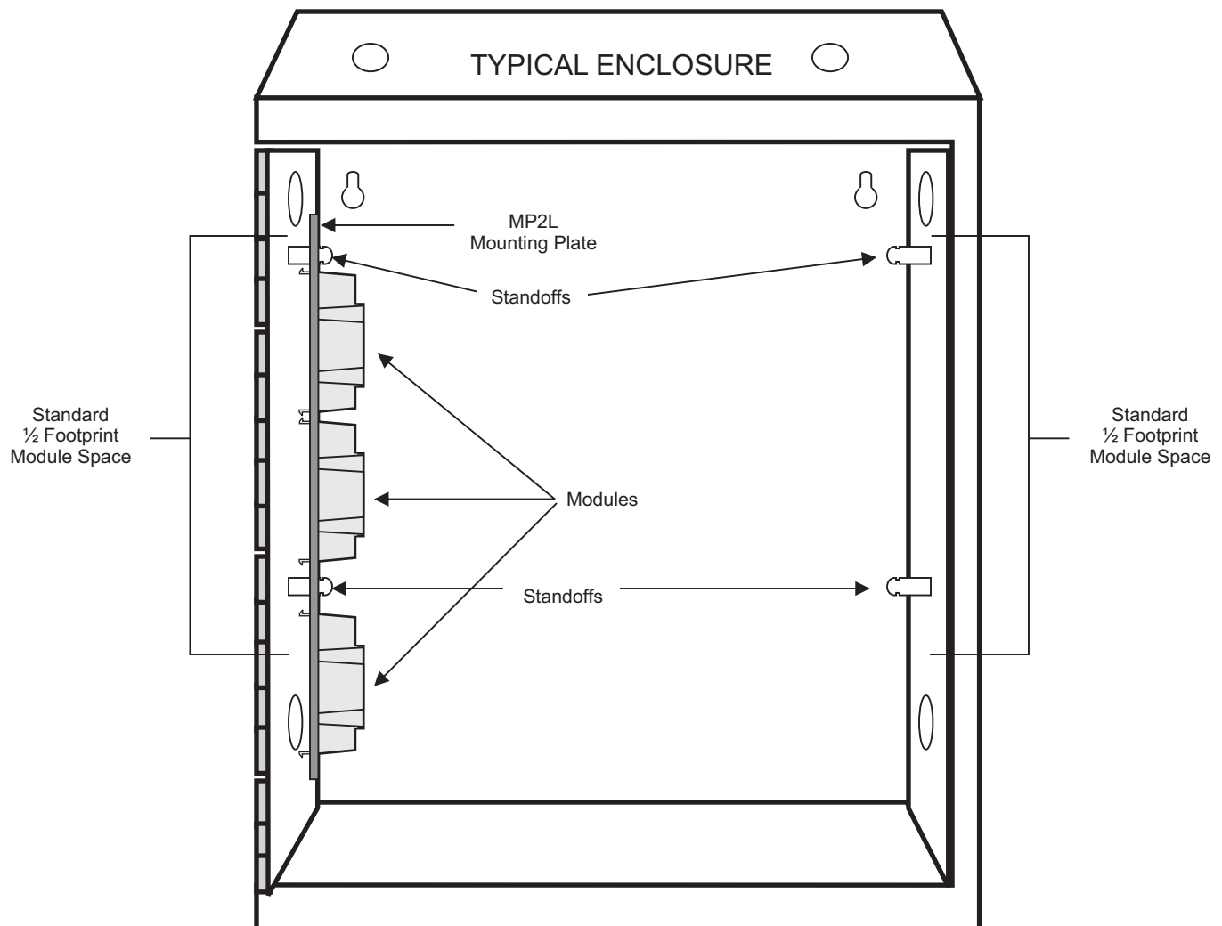
Figure 3, Mounting MP2L to Enclosure Standard ½ Footprint Module Space
