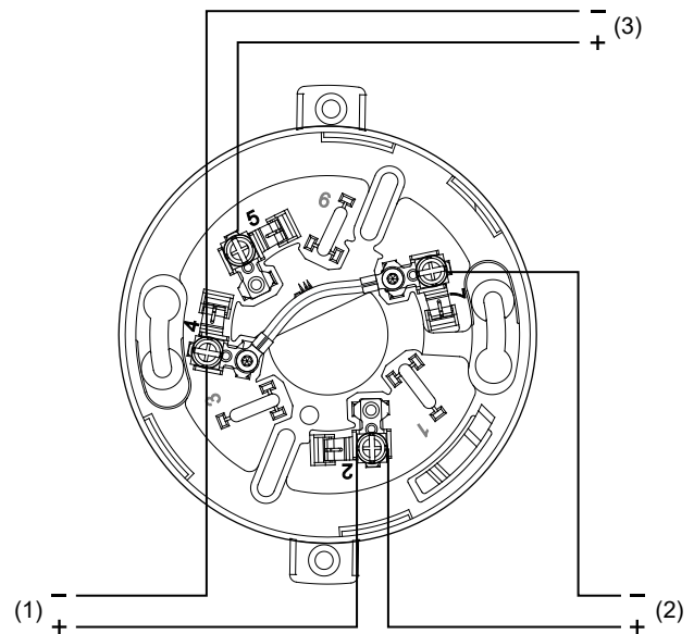
Figure 1: Wiring the detector base
